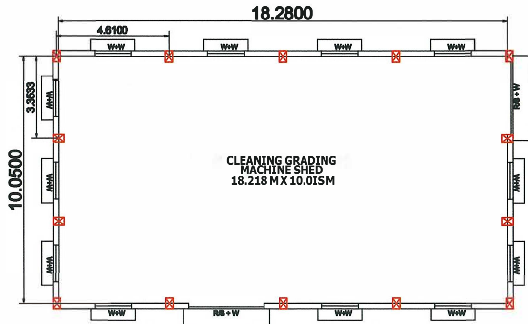
CLEANING GRADING MACHINE SHED scale 1:100 SIZE 18.28 M X 10.05 M X 10.05 M
